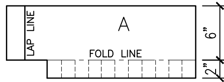
FINGER CUT
